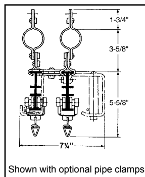
Cross Section of 420 Track at Center Overlap Pipe Mounted
