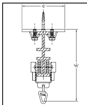
Cross Section of 422 Ceiling Mount
