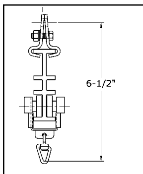
Cross Section of 422 Suspended
