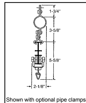
Cross Section of 422 Track Pipe Mounted
