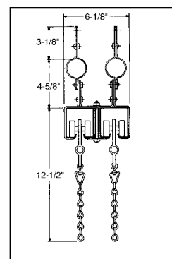
Cross Section of 280 Track at Center Overlap Pipe Mounted
